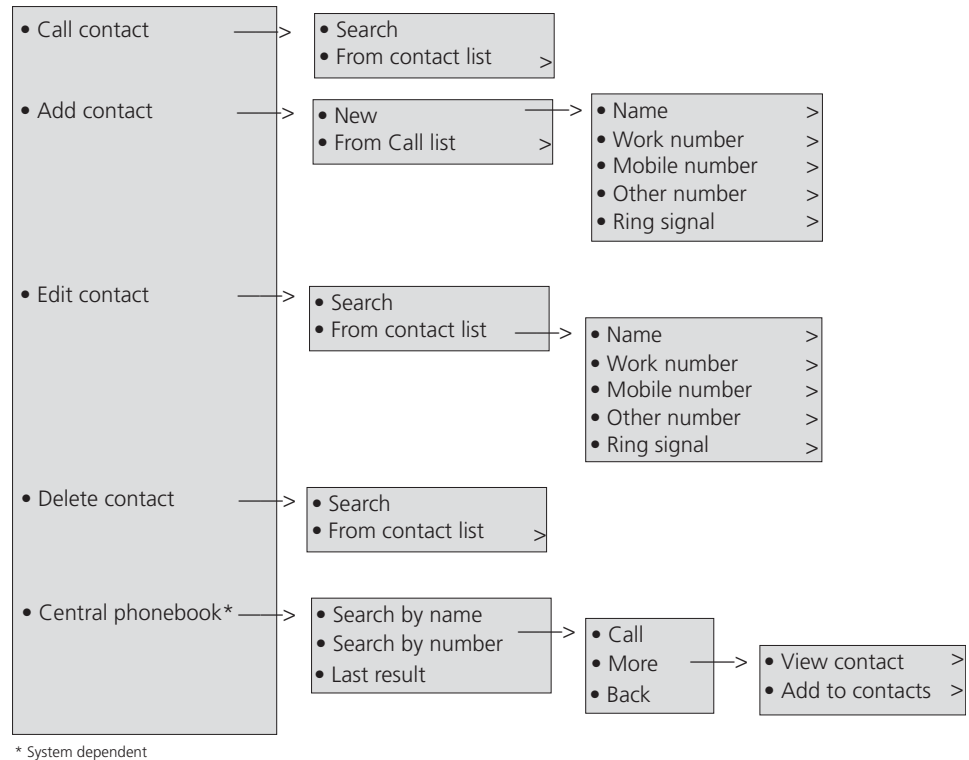
Figure 6: Contacts Menu
