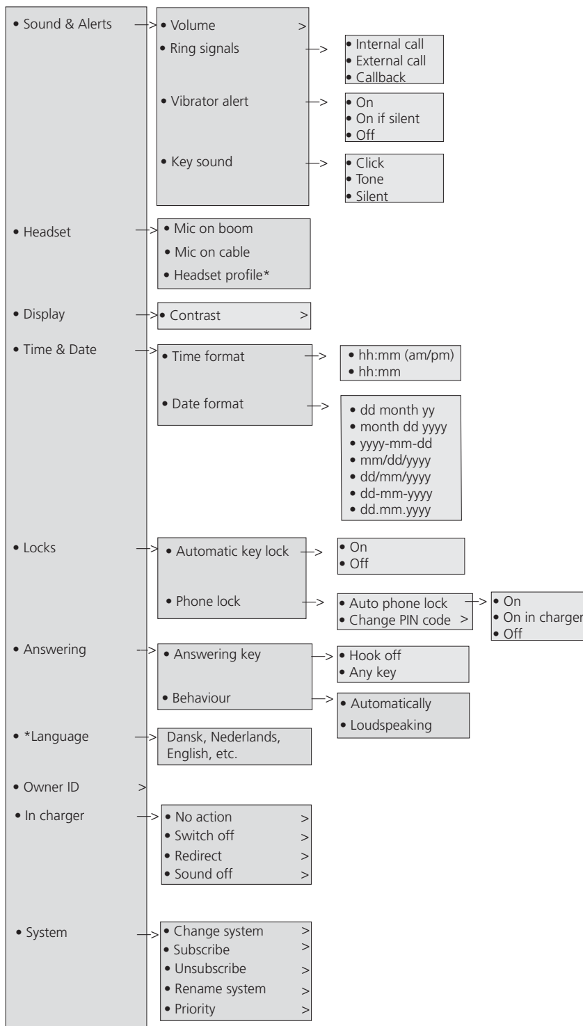
Figure 7: Settings Menu
